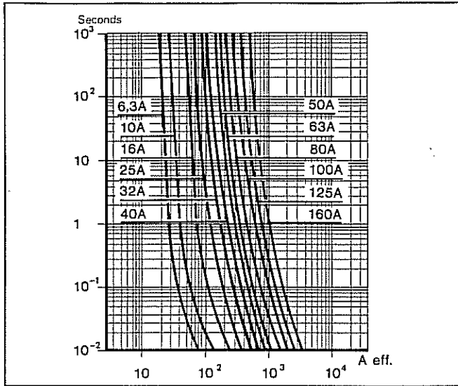
Time/current characteristics (pre-arcing duration)
