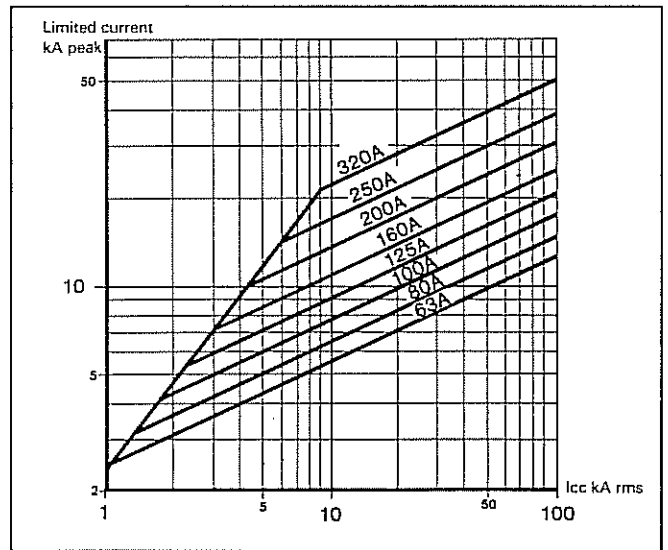
Cut-off current characteristics (limiting effect)
