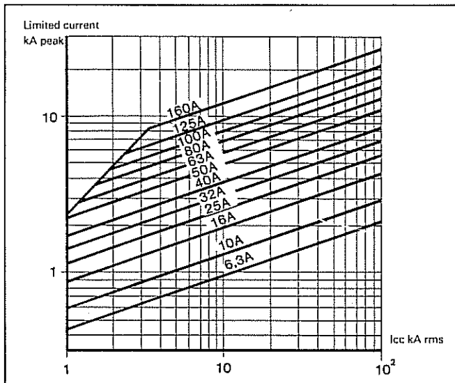
Cut-off current characteristics (limiting effect)
