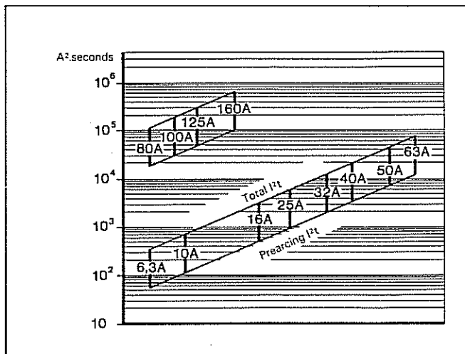
Joule integral, prearcing and total
