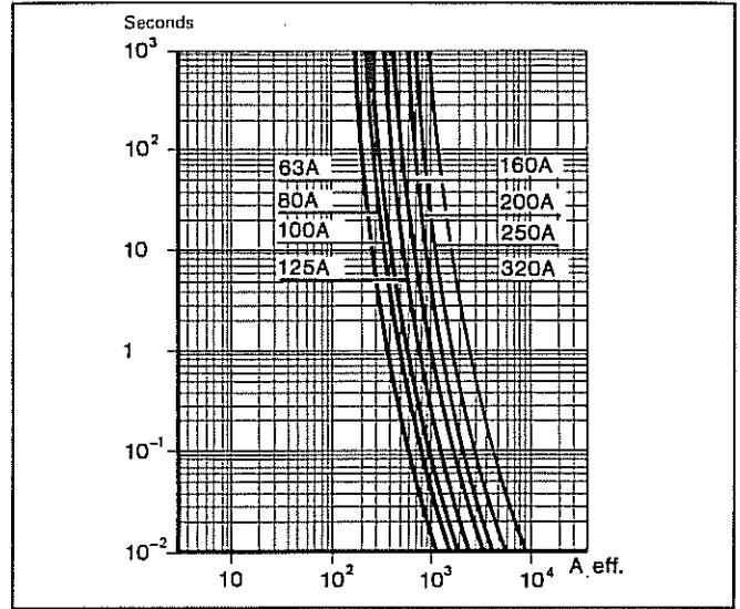
Time/current characteristics (pre-arcing duration)
