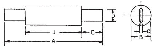
TYPE 3 70-600A
