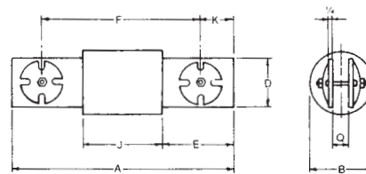
TYPE 4 650-1200A
