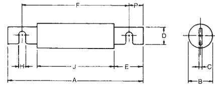
TYPE 4 70-600A
