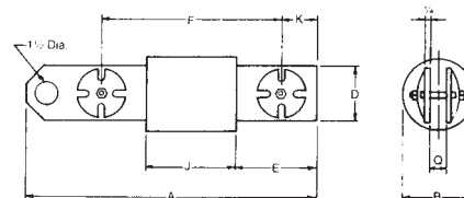
TYPE 5 650-1200A
