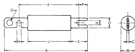
TYPE 5 125-600A
