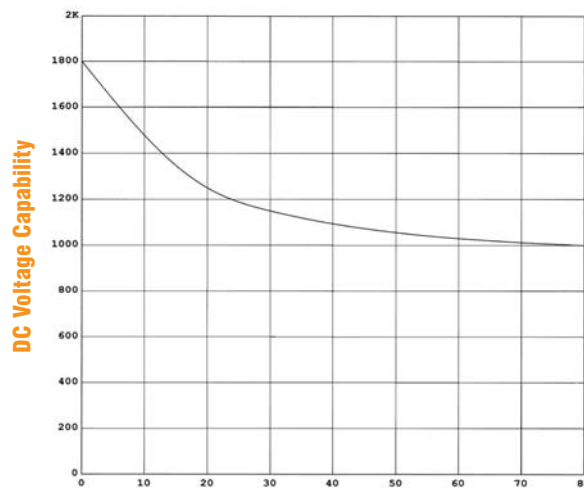
Circuit Time Constant L/R (ms)
