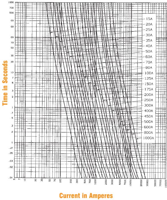
Melting Time – Current Data, 1500V Fuses
